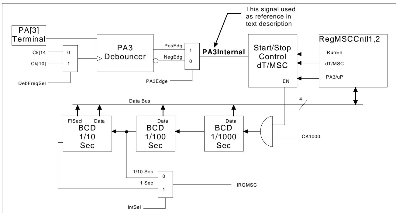
Figure 26. MSC Block Diagram
