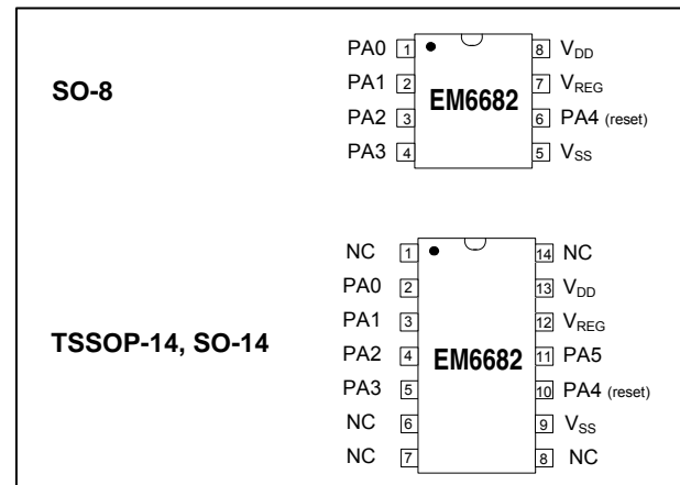
Figure 2. Pin Configuration
