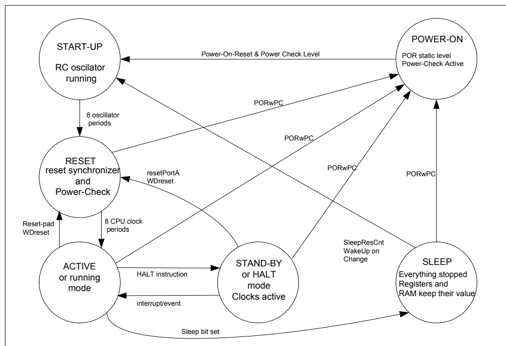
Figure 5. EM6682 operating mode transitions
