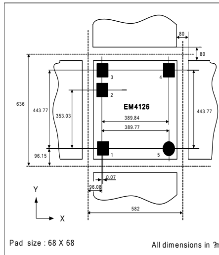
Fig. 4: Chip dimensions and pins locations
