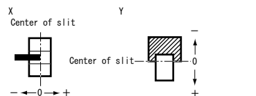
*2 Method of measuring position detection characteristic
