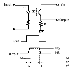
*1 Switching time measurement circuit
