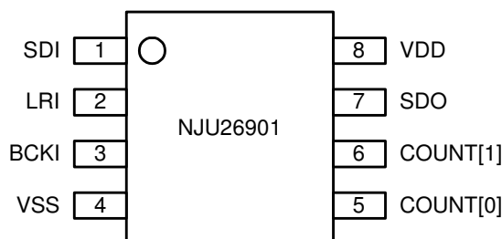
Fig. 2 Pin Assignment
