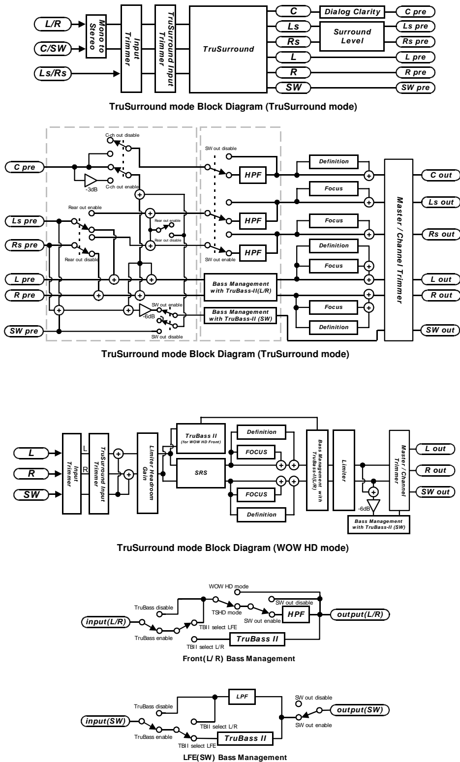
Fig.1-3c NJU26040-09D Function Diagram
