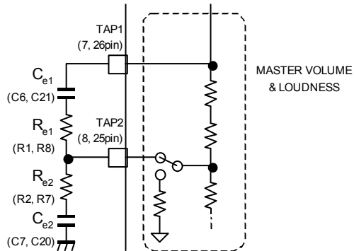
fig. A Loudness circuit
