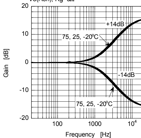
Gain vs Frequency (TONE Treble)
