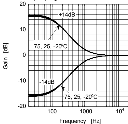
Gain vs Frequency (TONE Middle)
