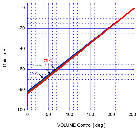
Gain vs VOLUME Control
