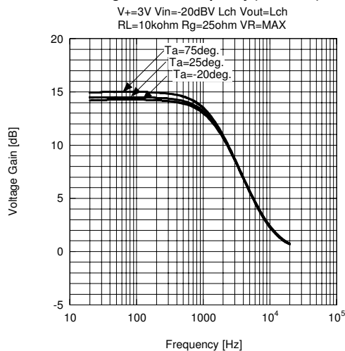
Voltage Gain vs. Frequency (Surround)
