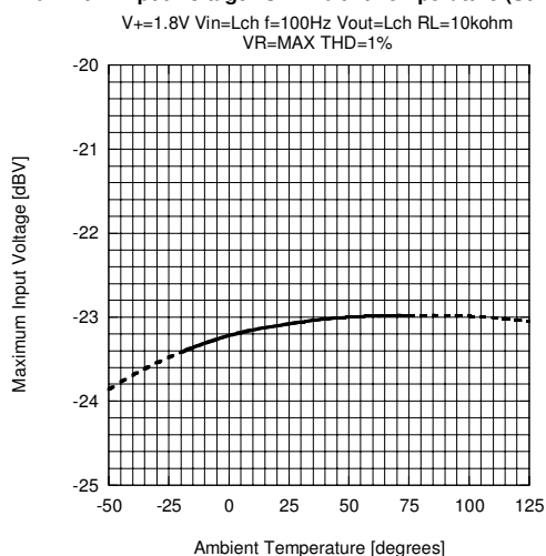
Maximum Input Voltage vs. Ambient Temperature (Surround)
