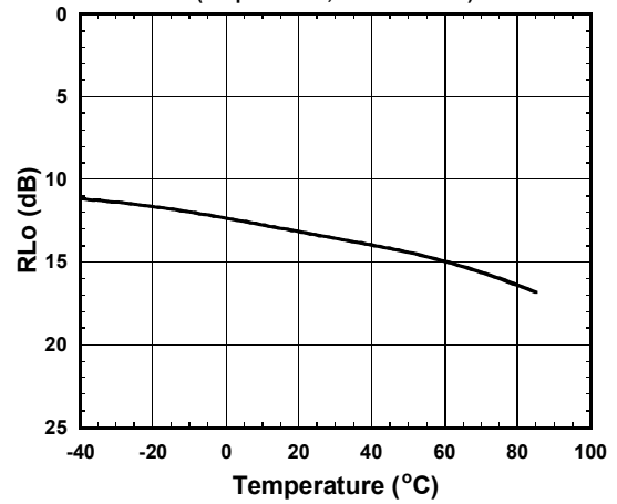
RF OUT Return Loss vs. Temperature (freq=620MHz, Z_s=Z_l=75\text{ohm} )
