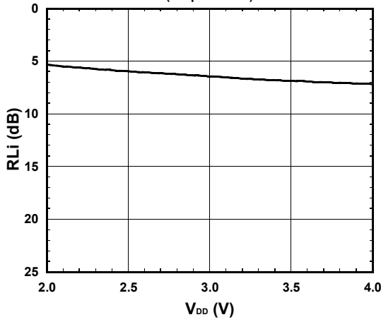
RF IN Return Loss vs. V_{DD} (freq=620MHz)
