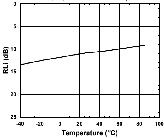
RF IN Return Loss vs. Temperature (freq=620MHz, Z_s=Z_l=75\text{ohm} )
