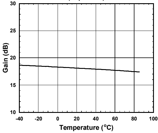
Gain vs. Temperature (freq=620MHz)
