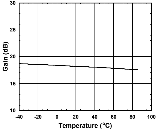
Gain vs. Temperature (freq=620MHz, Z_s=Z_l=75\text{ohm} )
