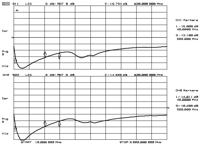
S11, S22
