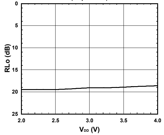
RF OUT Return Loss vs. V_{DD} (freq=620MHz)
