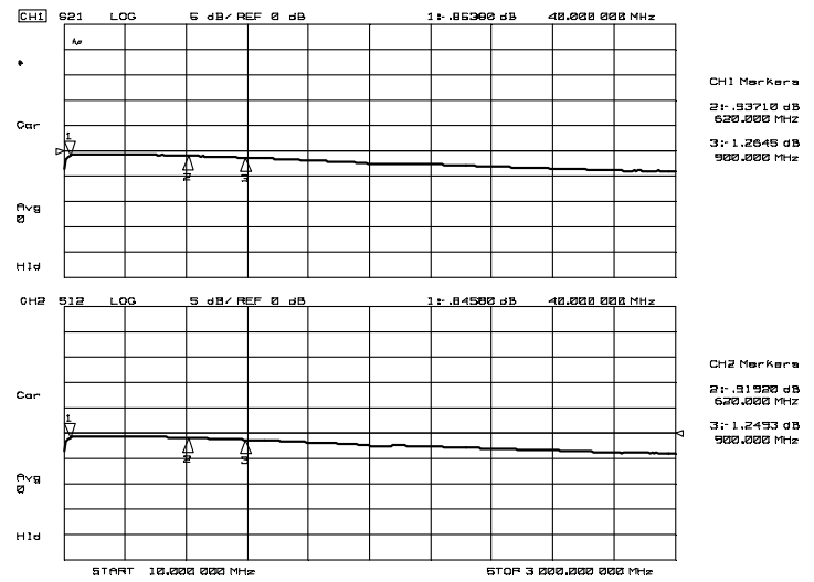
S21, S12 (f=10MHz~3GHz)
