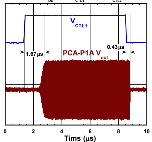
Switching Time
