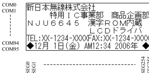
The correspondence of the display position on the panel and the DDRAM address (SEL1="1", SEL2="0")
