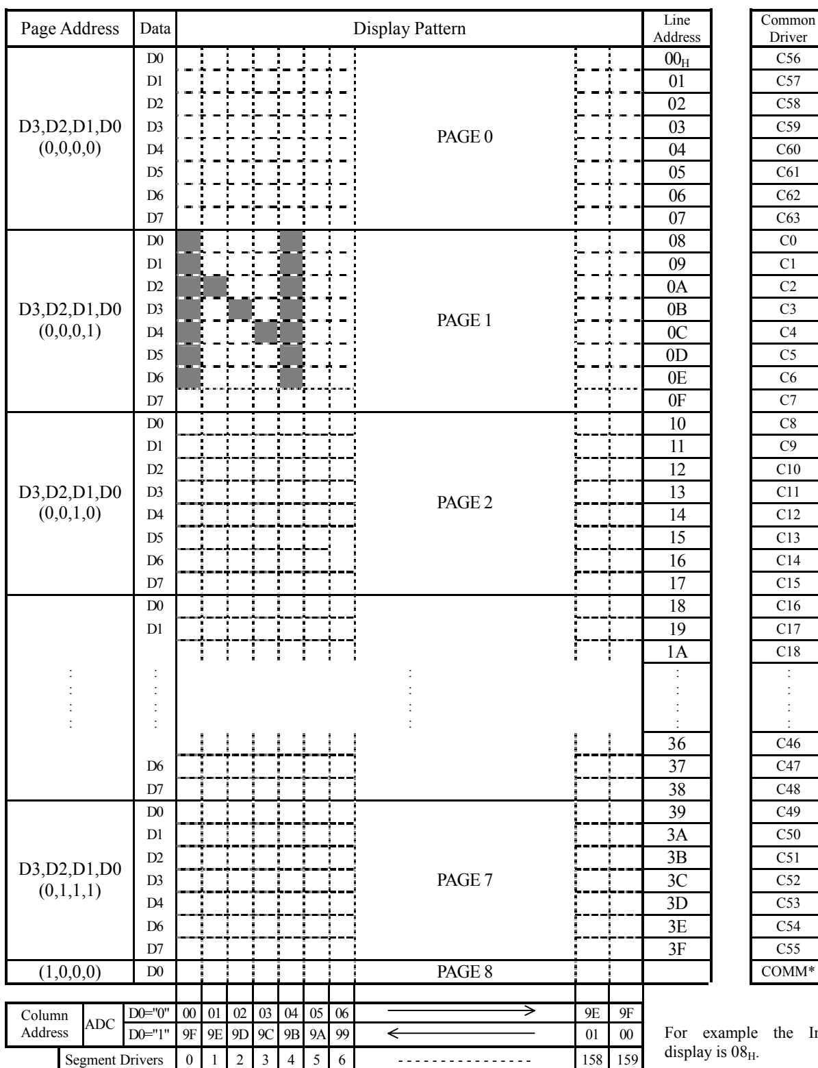
Fig.1 Display data RAM (DDRAM) Map
