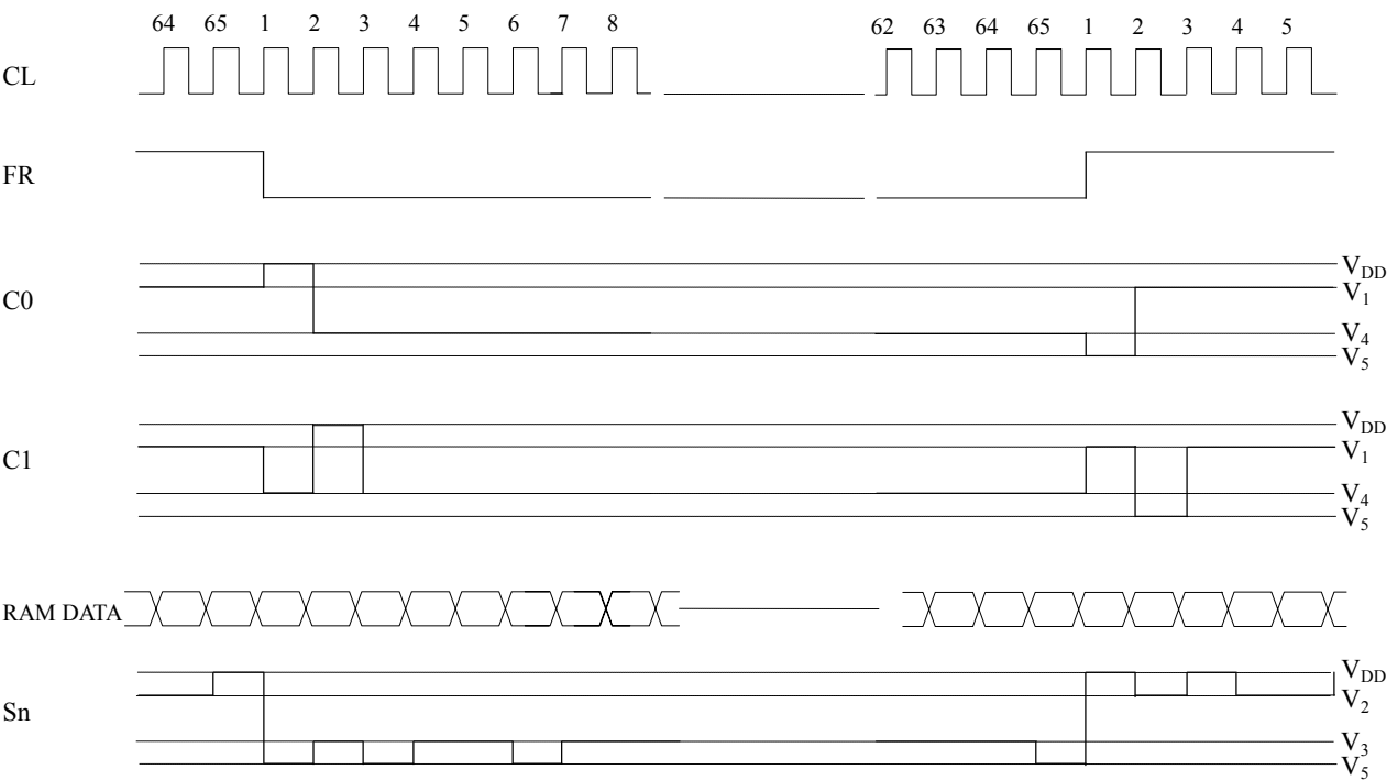
(e) Common timing generation The common timing is generated by display clock CL (refer to Fig.2)
