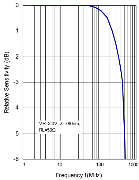
Relative Sensitivity vs. Frequency ( T_a=25^\circ\text{C} )
