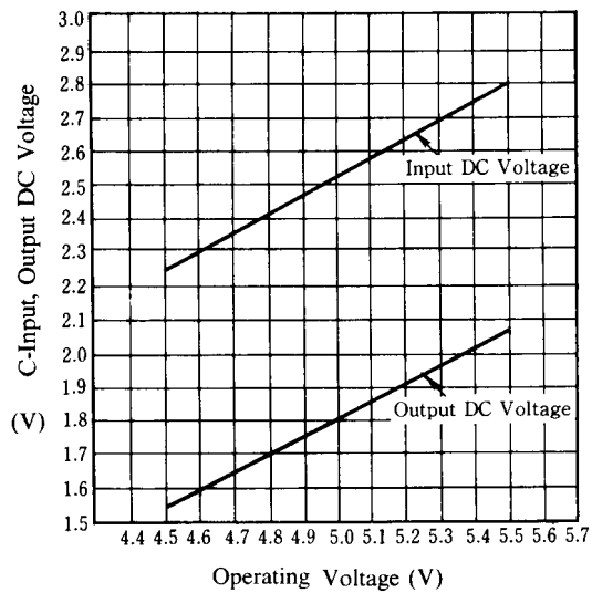
C-Input, Output DC Voltage vs. Operating Voltage
