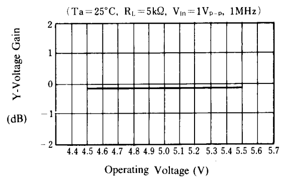
Y-Voltage Gain vs. Operating Voltage
