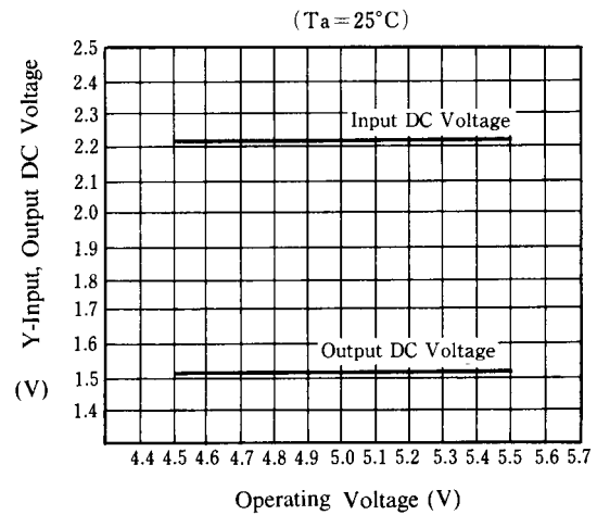
Y-Input, Output DC Voltage vs. Operating Voltage
