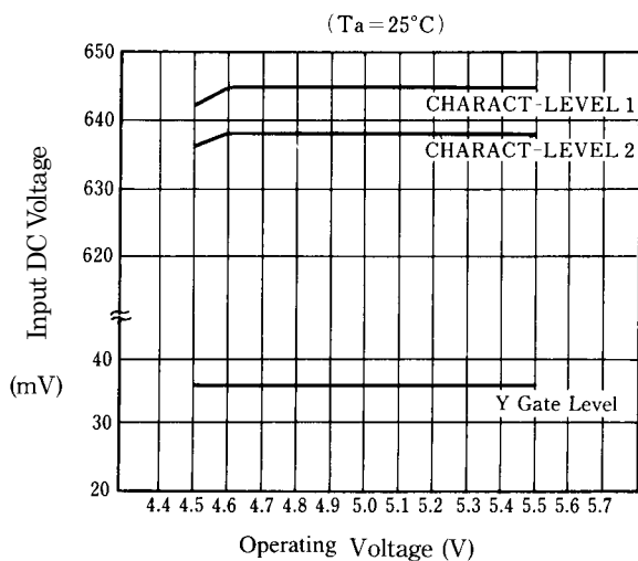
Input DC Voltage vs. Operating Voltage
