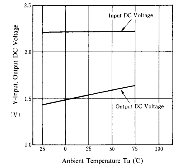
Y-Input, Output DC Voltage vs. Ambient Temperature
