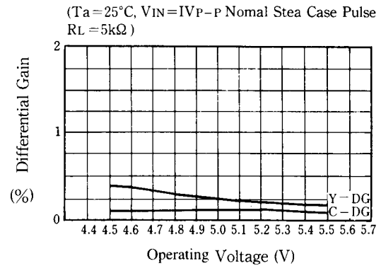
Differential Gain vs. Operating Voltage
