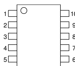
NJW1352KK1 (SON10)
