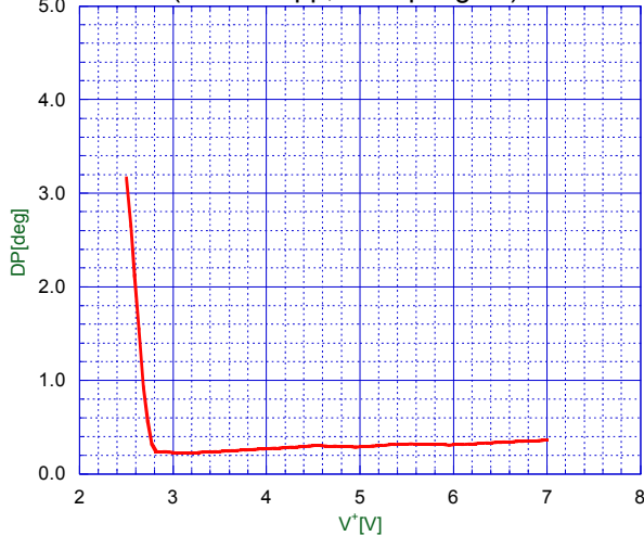
Differential Phase vs. Supply Voltage ( v_{in}=0.5\text{Vpp}, 10\text{Step-signal} )
