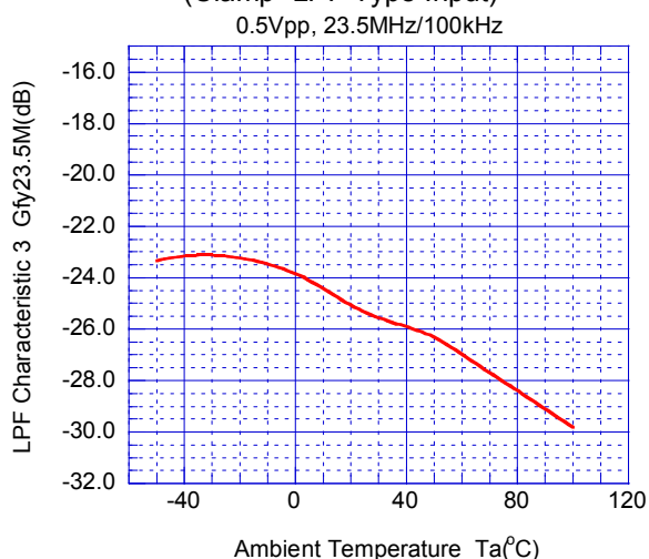
Low Pass Filter Characteristic 3 vs. Temperature (Clamp+LPF Type Input)
