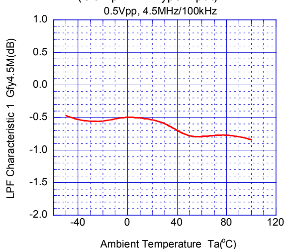
Low Pass Filter Characteristic 1 vs. Temperature (Clamp+LPF Type Input)
