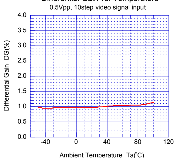
Differential Gain vs. Temperature
