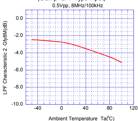
Low Pass Filter Characteristic 2 vs. Temperature (Clamp+LPF Type Input)
