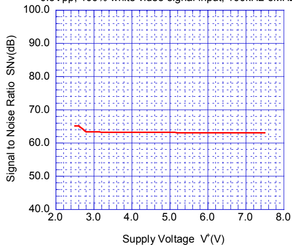
Signal to Noise Ratio vs. Supply Voltage 0.5Vpp, 100% white video signal input, 100kHz-6MHz
