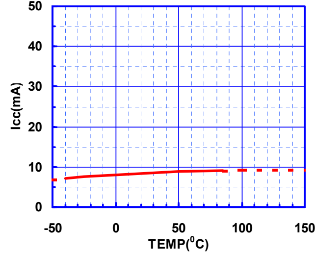
ICC vs Temperature
