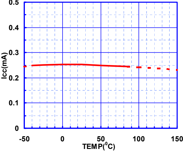
Isave vs Temperature
