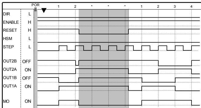
Fig.7 Full Step Mode / Reset Sequence
