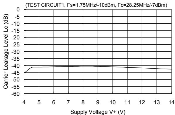
Carrier Leakage Level versus Supply Voltage
