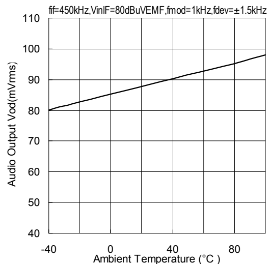
Audio Output versus Temperature
