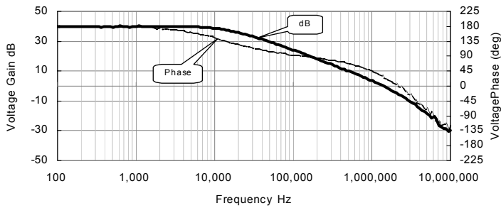
Ach Voltage Gain , Phase vs. Frequency Characteristic (V+=5V, Ta=25°C)
