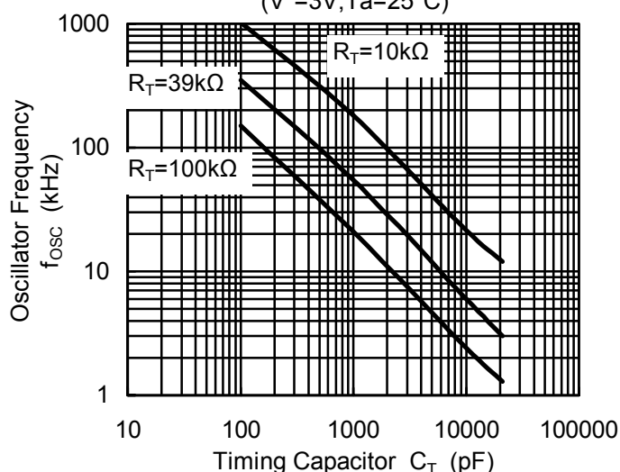
Oscillator Frequency vs. Timing Capacitor ( V^+=3V, T_a=25^\circ C )
