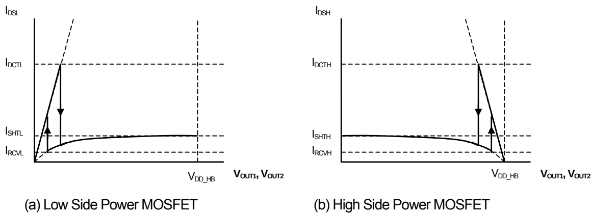
Fig. 2. Output Current Limit Circuit
