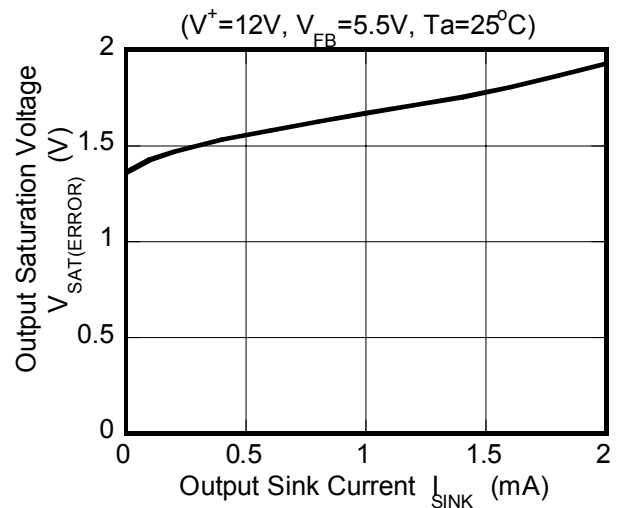
Error AMP Block Output Saturation Voltage vs. Output Sink Current
