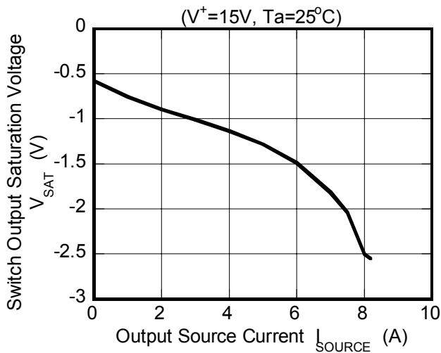
Switch Output Saturation Voltage vs. Output Source Current
