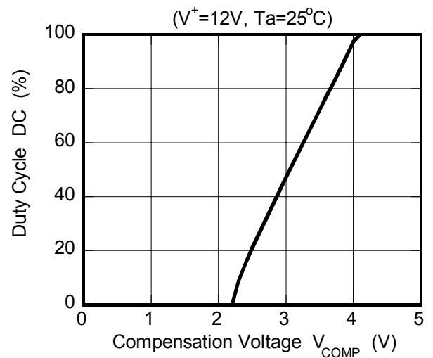
Duty Cycle vs. Compensation Voltage
