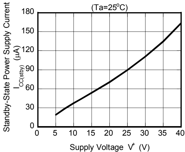
Standby-State Power Supply Current vs. Supply Voltage
