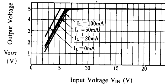
Output Voltage
