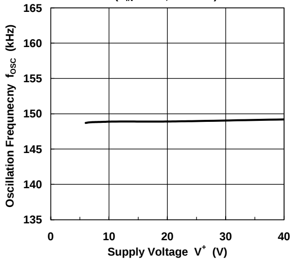
Oscillation Frequency vs. Supply Voltage ( V_{IN}=0.7V , T_a=25^\circ C )
