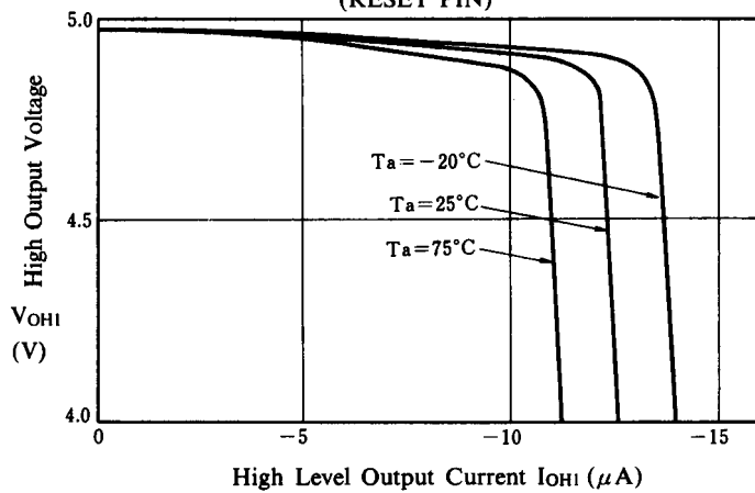
High Level Output Voltage vs. High Level Output Current (RESET PIN)
