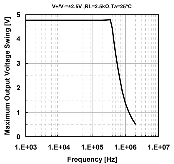
Maximum Output Voltage Swing vs. Frequency
