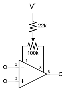
Fig.1-1 Input Offset Voltage Adjustment
