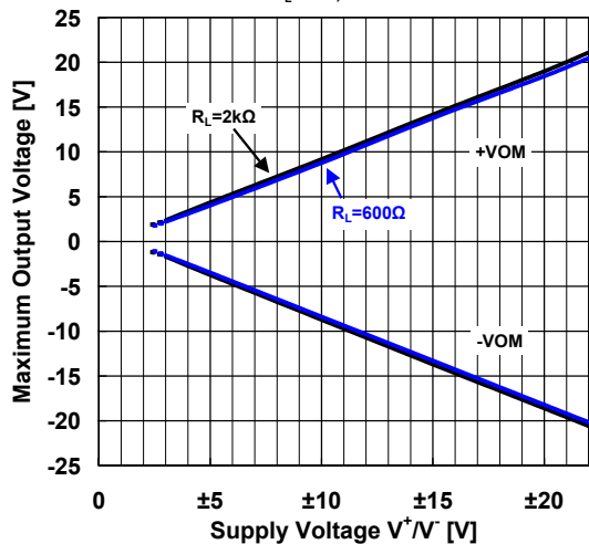
Maximum Output Voltage vs. Supply Voltage R_L=2\text{k}\Omega , T_a=25^\circ\text{C}
