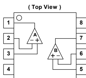
NJM14558D/14558M/14558E NJM14558V/14558R
