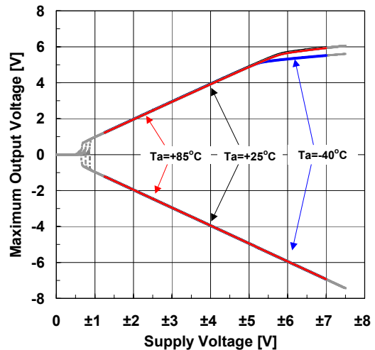
Maximum Output Voltage vs. Supply Voltage (Temperature, R_L=5k\Omega ) G_V=OPEN, R_L=5k\Omega
