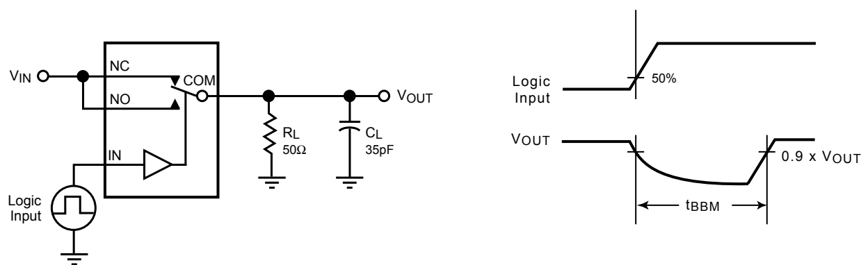
Figure 3. Break Before Make Interval Timing
