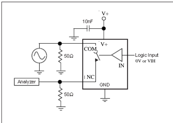
Figure 4. Off Isolation
