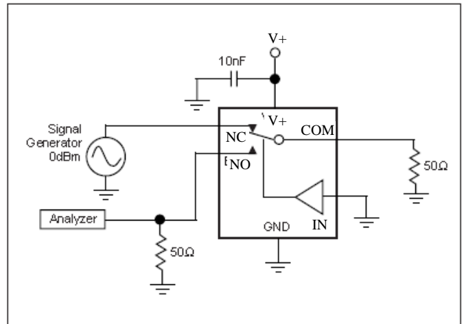
Figure 5. Crosstalk
