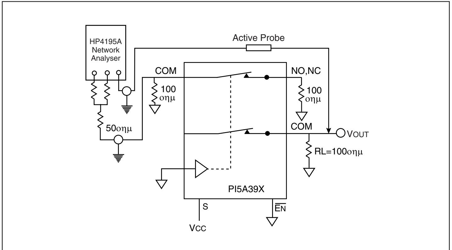
Figure 4. Crosstalk
