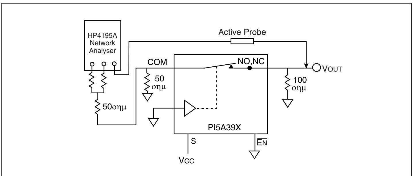
Figure 5. Off Isolation
