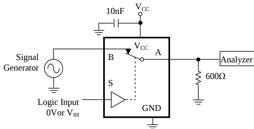
Figure 7. Harmonic Distortion
