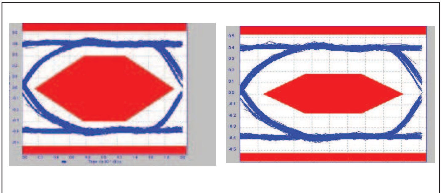
Figure 2: USB 2.0 High Speed (480Mbps) TP1, left eye, and TP5, right eye, with PI3USB102A in the signal path while HDD is driving.
