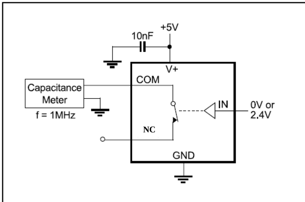
Figure 4. Channel-On Capacitance
