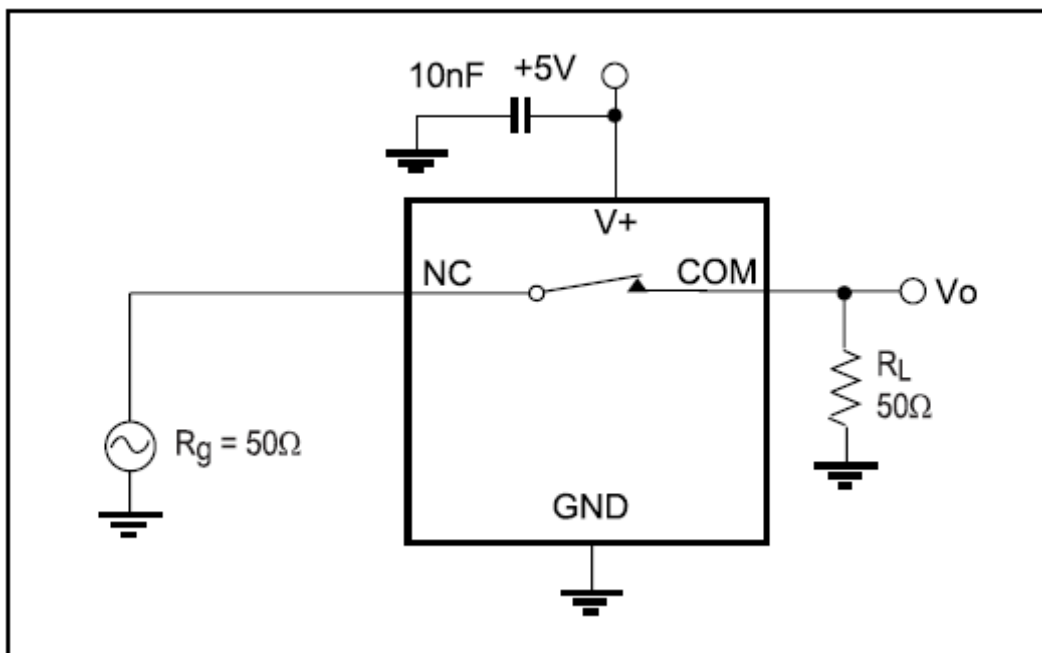
Figure 5. Bandwidth
