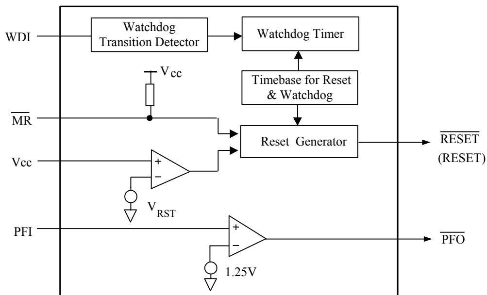
PT7M7823/24/25 Block Diagram
