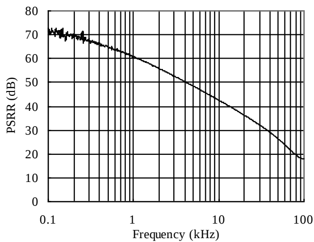
PT7M8220B (3.3V) Vin=4.3V DC+1Vp-pAC Cout=1uF(Ceramics), Iout=30mA
