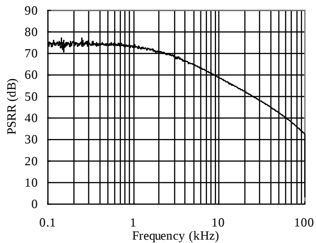
PT7M8220B (1.2V) Vin=2.2V DC+1Vp-pAC Cout=1uF(Ceramics), Iout=30mA
