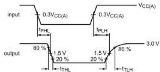
Figure 3: Propagation Delay and Transition Times A→B
