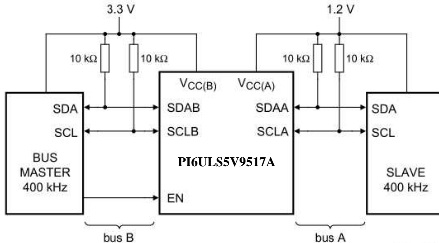
Figure 6: Typical Application
