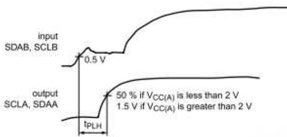
Figure 4: Propagation Delay
