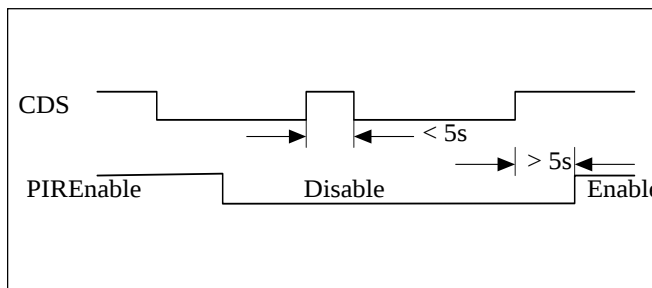
Figure 4. CDS Enable Debounce
