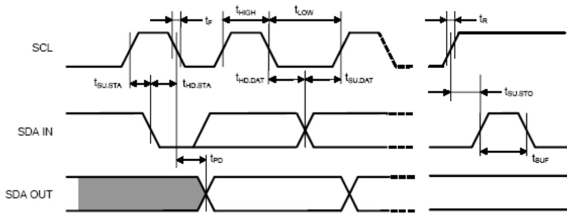
Timing Chart
