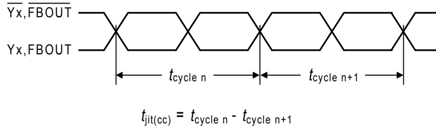
Figure 3. Cycle-to-Cycle Jitter
