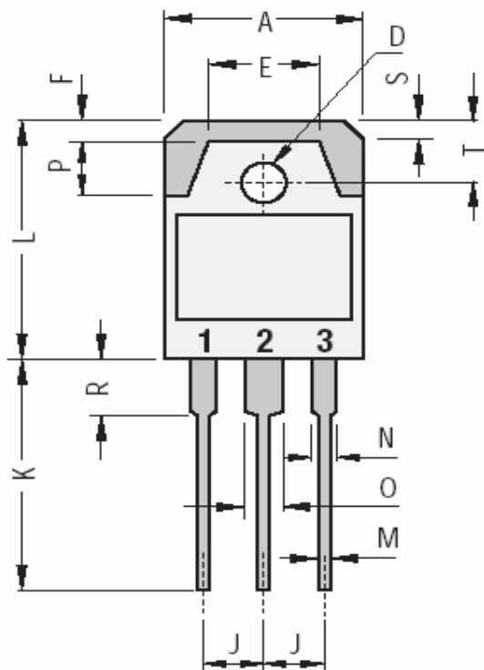
TO-3PN Non Isolated Leaded Plastic Package
