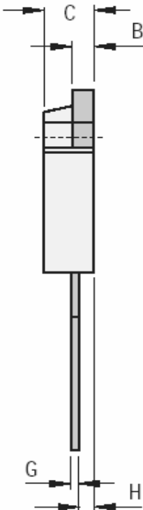
TO-3PN Non Isolated Leaded Plastic Package
